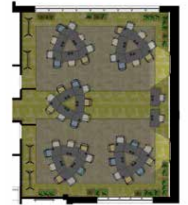
Conference cluster 2
