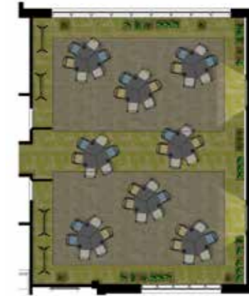
Conference cluster 1
